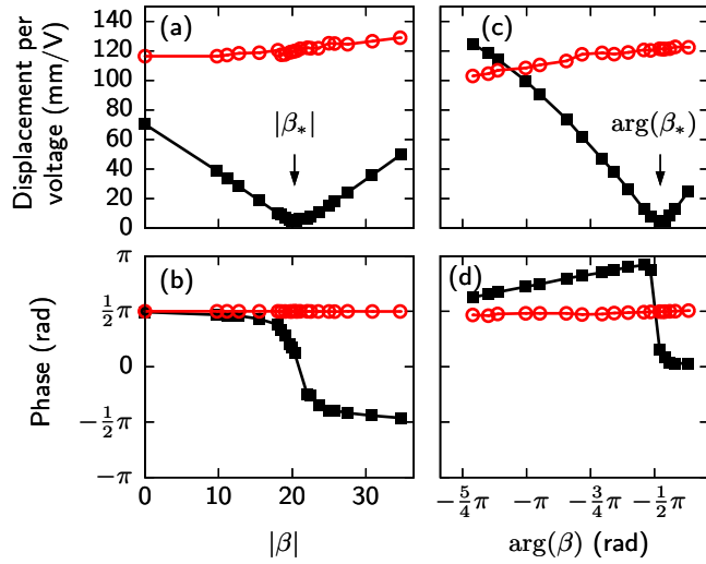
FIG. 6: Adjusting unidirectionality. Unidirectionality emerges when the ratio \beta of the piezoelectric-element voltage to the coil voltage, \beta \equiv \tilde{V}_p/\tilde{V} , which relates linearly to the coefficient \alpha , is tuned to the critical value \beta_* of the correct amplitude and phase. We show the diaphragm displacement per coil voltage, \tilde{X}_d/\tilde{V} (black squares) as well as the coil displacement per coil voltage, \tilde{X}_c/\tilde{V} (red circles) that result when the coil but not the diaphragm is stimulated. (a),(b), The amplitude and phase of the displacement per voltage when the magnitude of \beta is varied and its phase is held constant at the critical value |\beta_*| . (c),(d), The amplitude and phase of the displacement per voltage when the phase of \beta is varied and its magnitude held constant at the critical value |\beta_*| . The coil's displacement per voltage is largely independent of \beta (a,b,c,d). However, the diaphragm's displacement almost vanishes at \beta_* , showing that the forces on the coil are not transmitted to the diaphragm and thus demonstrating unidirectionality (a,c). The diaphragm's displacement does not vanish completely at \beta_* because of nonlinearities in the piezoelectric element and because of noise. In agreement with theoretical analysis, the diaphragm's displacement undergoes a phase change of \pi around \beta_* (b,d).
