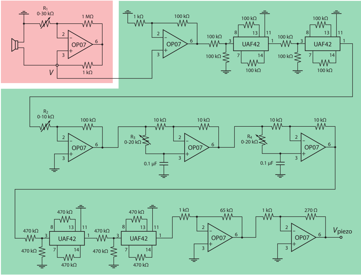
FIG. 4: Electrical circuit. The electrical circuit indicated in red provides positive feedback for mechanical amplification in the microphone and constitutes the circuit indicated in red in Fig. 1(d),(e). Its feedback gain can be adjusted by varying the resistance R_1 . The circuitry indicated in green converts the coil voltage V into a voltage V_{\text{piezo}} that is fed into an amplifier of maximal voltage 150 V and gain 10\times to yield the piezo voltage V_p . The gain of this circuit can be controlled through the variable resistance R_2 and its phase through the variable resistances R_3 and R_4 . Four two-pole low-pass filters are constructed with the help of filters (UAF42; Texas Instruments). This arrangement constitutes the circuit indicated in green in Fig. 1(e).
