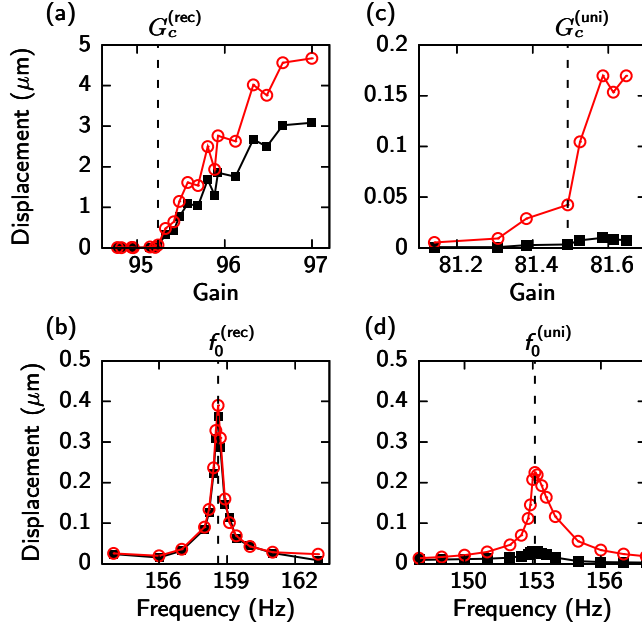
FIG. 5: Hopf bifurcation. We show the displacement of the coil (red circles) and of the diaphragm (black squares) for the reciprocal active (a,b) and the unidirectional active microphone (c,d). (a),(c), The reciprocal active and the unidirectional active microphone exhibit supercritical Hopf bifurcations at the critical values G_c^{(\text{rec})} \approx 95.2 and G_c^{(\text{uni})} \approx 81.5 of the gain in amplifier A . In the absence of an external stimulus, and apart from noise, the system is quiescent below G_c . For gains exceeding G_c spontaneous limit-cycle oscillations emerge in the coil. The diaphragm displacement reflects the Hopf bifurcation in the reciprocal but not in the unidirectional system. (b),(d), When operating at the Hopf bifurcation and stimulated by sound of different frequencies at a constant sound-pressure level of 60 dB SPL, the responses of the reciprocal and the unidirectional active microphones are tuned sharply around their resonant frequencies of f_0^{(\text{rec})} \approx 158.6 Hz and f_0^{(\text{uni})} \approx 153.1 Hz. The diaphragm's motion approximately equals the coil's motion in the reciprocal microphone, but is much smaller than the coil's displacement in the unidirectional system.
